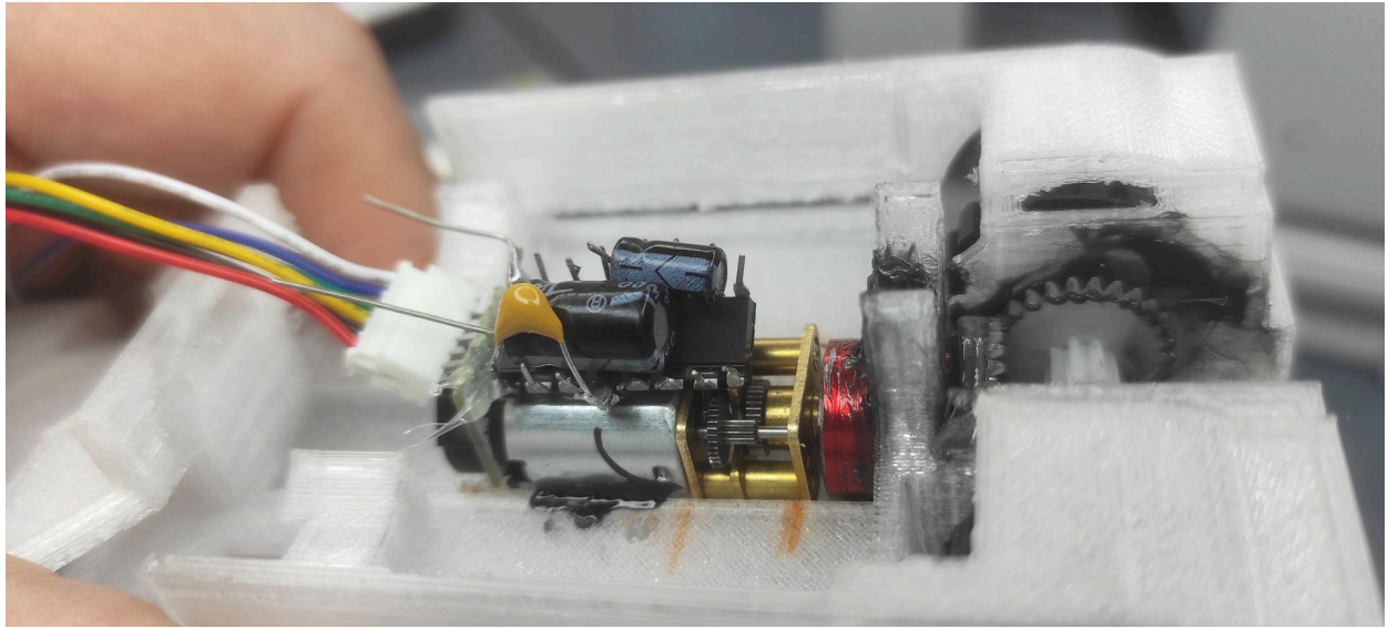
Motor driver and motor assembled into a single conjoined unit
