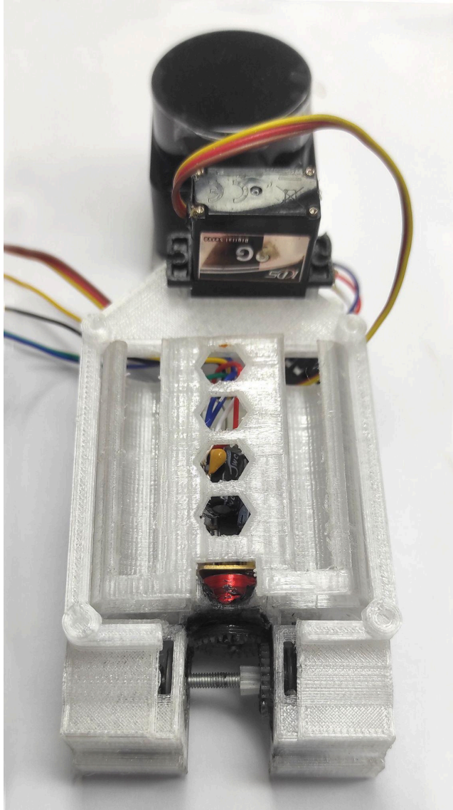
Steering servo and LiDAR placed
