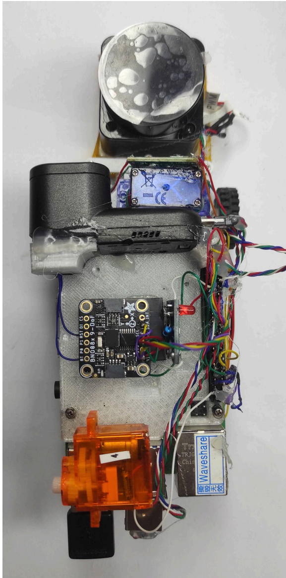
Full assembly including wiring completed
