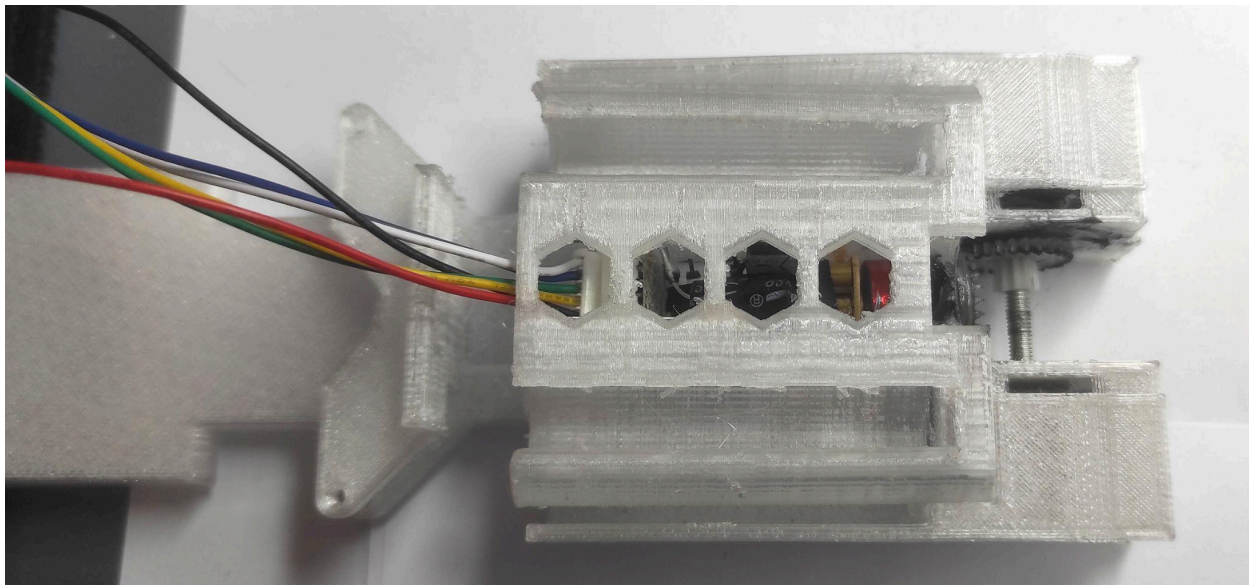
Motor driver and drive system fully assembled and enclosed with housing
