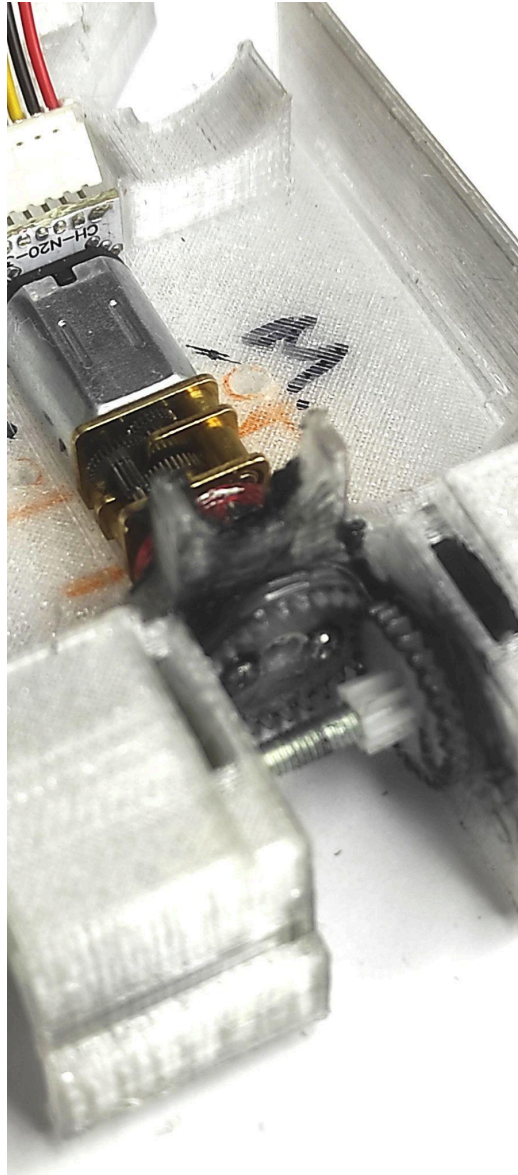
Drive motor and transfer gear fully assembled and tested
