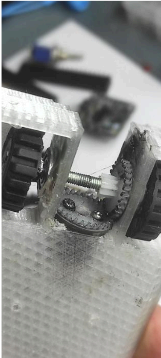
Drive shaft and transfer gear fully fitted
