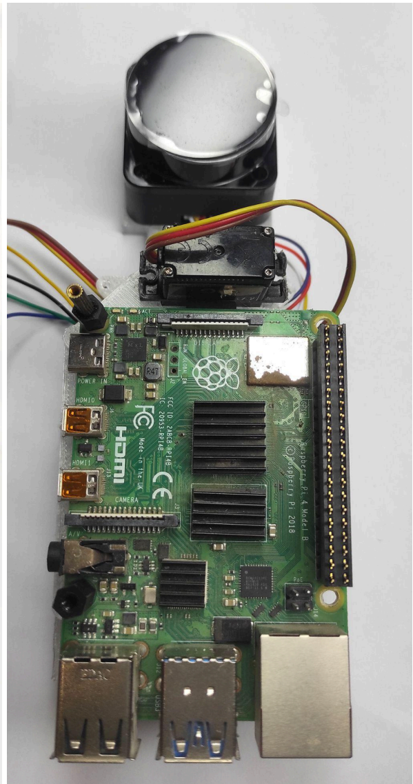
Raspberry Pi fitted on housing
