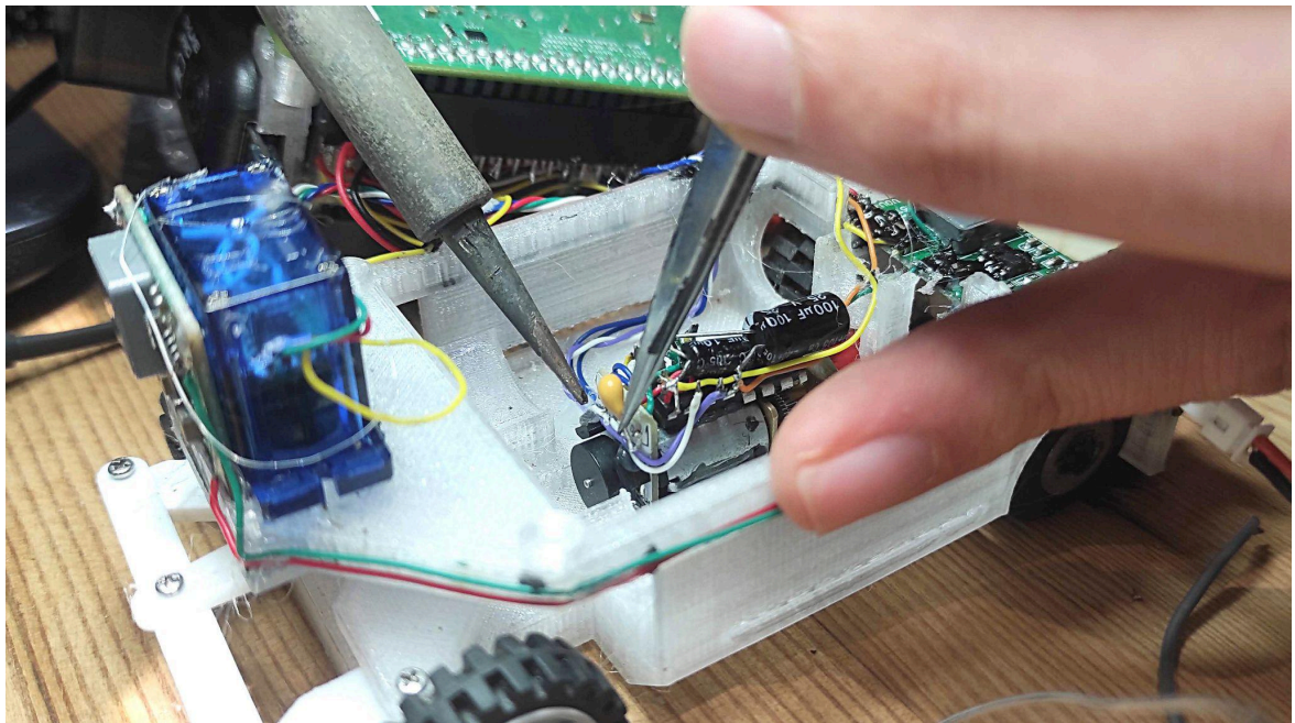
Soldering wires to the motor and motor driver
