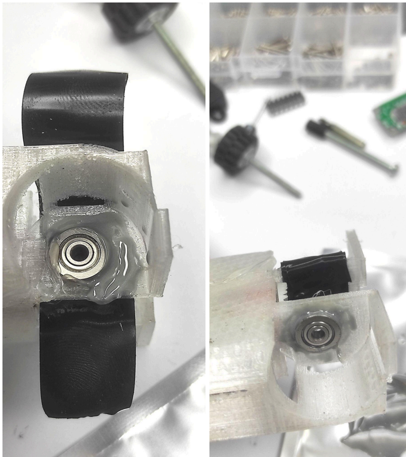
Wheel bearing fitted and glued
