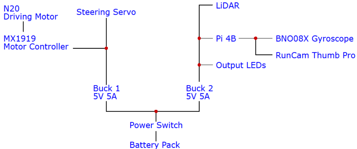
Power Distribution map
