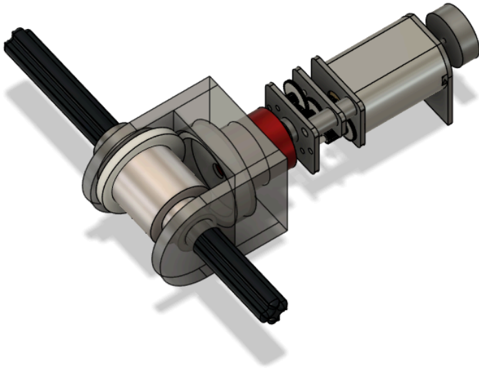
CAD Model of the complete motor-gearbox-axle assembly
